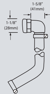
Overflow Assembly E52-1000
