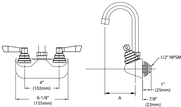
Swivel Gooseneck
